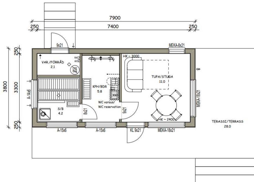
TeriMODULAR - SANDVIK SAUNA 30
